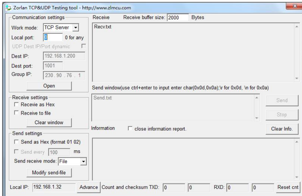
Figure 10 SocketTest Send-receive Interface
