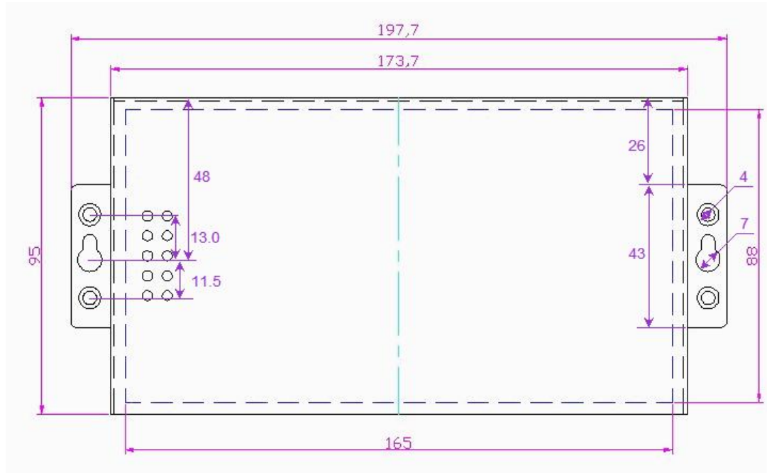
Chart 36 ZLAN5443H mounting size
