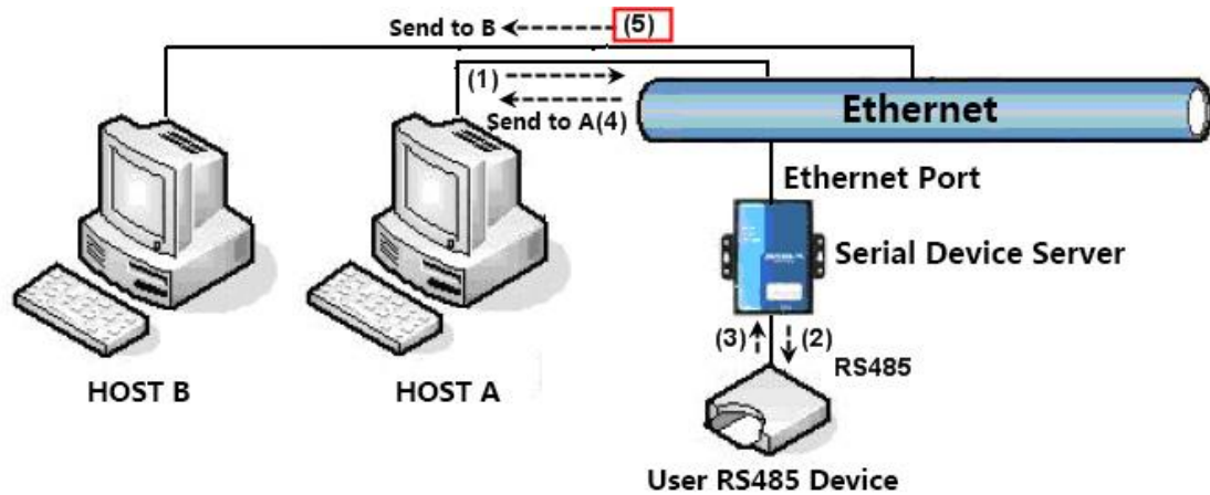
Chart 28 multi-host function demo
