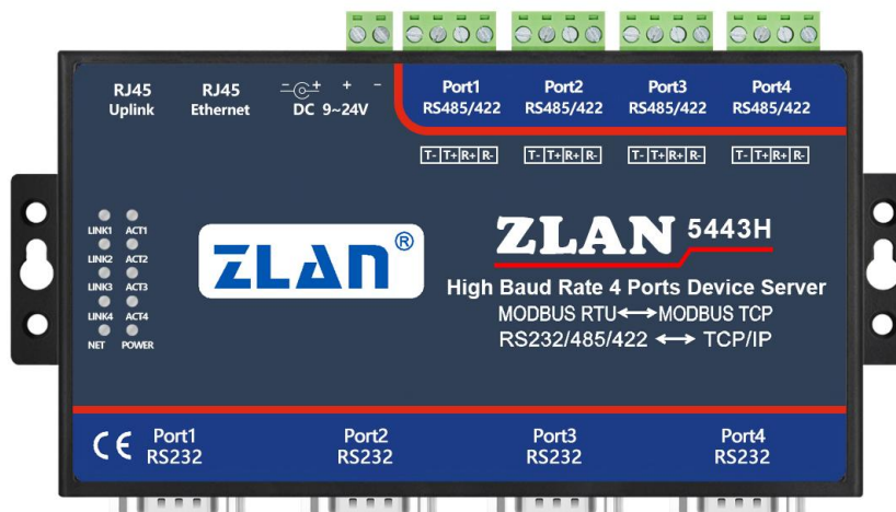
Chart 2 ZLAN5443H Front view
