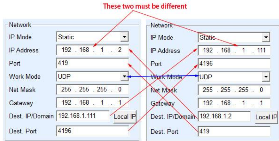
Chart 22 configuration of UDP device pairing parameters
