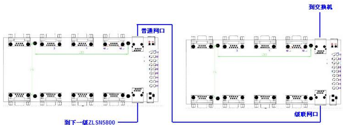
Chart 36 ZLAN5843A Cascade method
