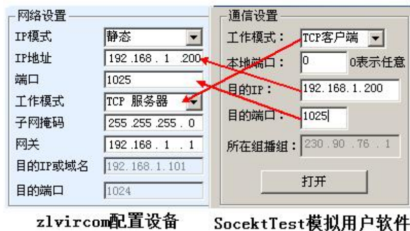
Chart 19 serial server being service terminal
