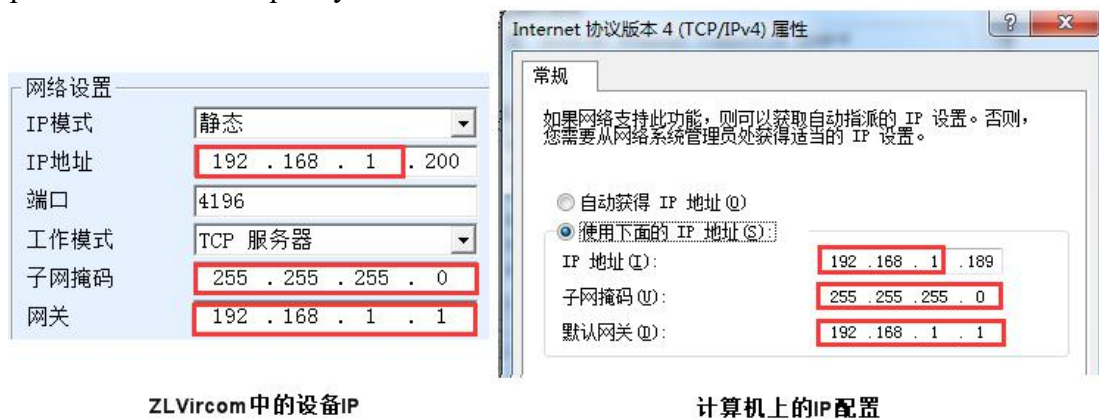
Chart 24 Configured on the same network segment
