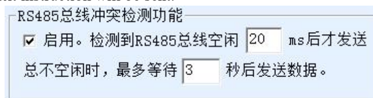
Chart 31 RS485 collision proof idle time
