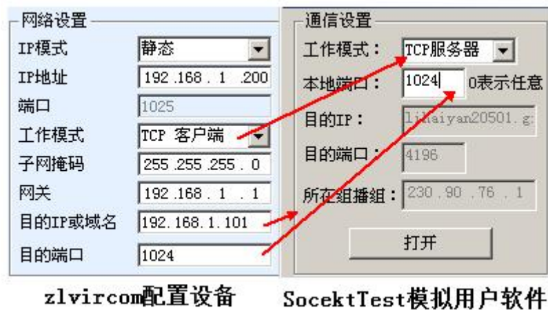
Chart 18 serial server being client terminal
