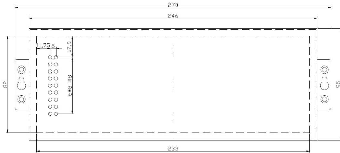
Chart 37 ZLAN5843A mounting dimension
